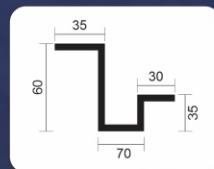
Talang Rembes Tipe U
