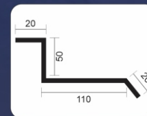
Talang Rembes Tipe Z
